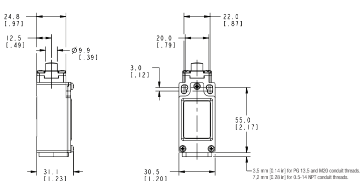
Figure 6. GLC Top Pin Plunger
