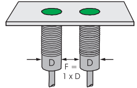
Flush installed proximity sensors, F must be equivalent to the housing diameter
