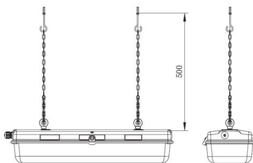
Chain mounting
