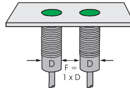
Flush installed proximity sensors, F must be equivalent to the housing diameter
