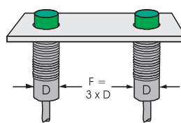
Non-flush installed proximity sensors, F must be 3 times the housing diameter
