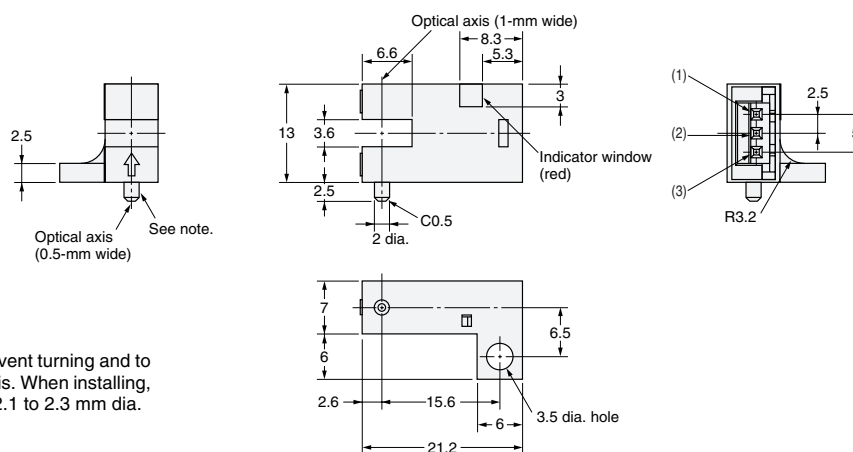
Terminal Arrangement
