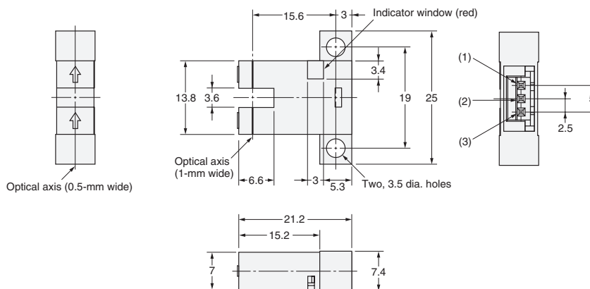
Terminal Arrangement
