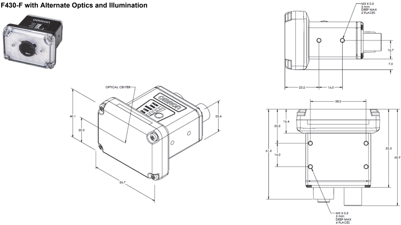
F430-F with Alternate Optics and Illumination
