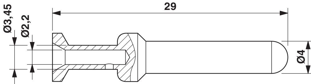
Dimensional drawing
