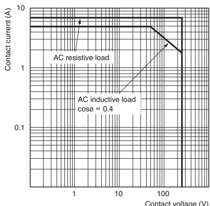
MY4□□-□□-GS (AC load)
