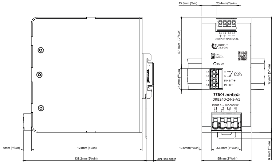
Fig. 18: Dimension drawing of DRB240-24-3-A1
