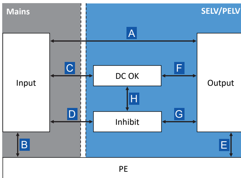
Fig. 24: Schematic of the insulation paths
