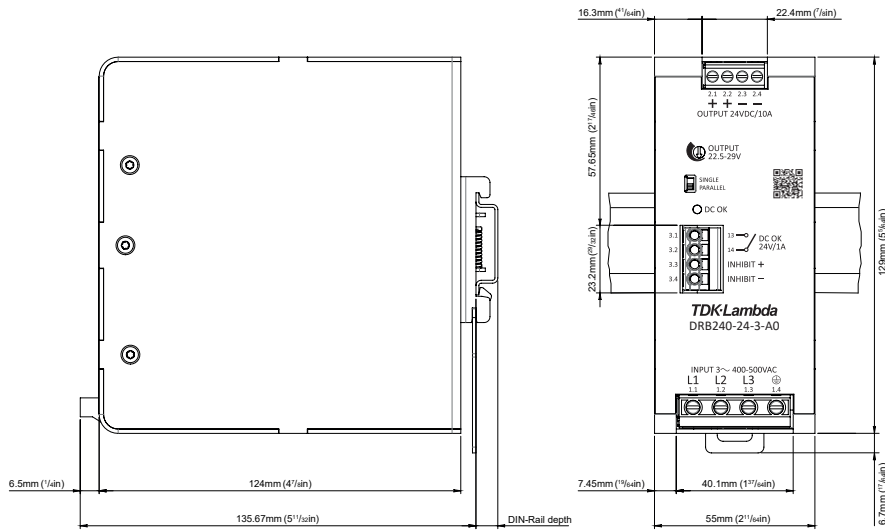
Fig. 17: Dimension drawing of DRB240-24-3-A0
