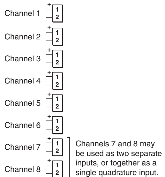
Fig 3 Input terminals
