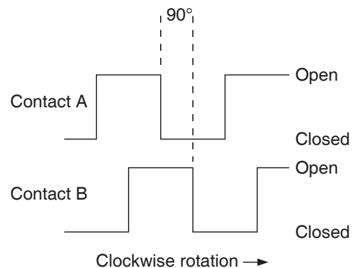
Fig 6 Quadrature sensor waveforms
