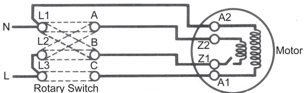
Connection diagram for utilising a three phase reversing switch for a single phase motor.
