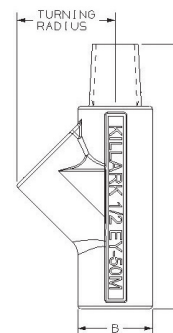
EY with Nipple Male to Female
