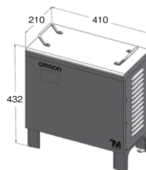
Control Box
