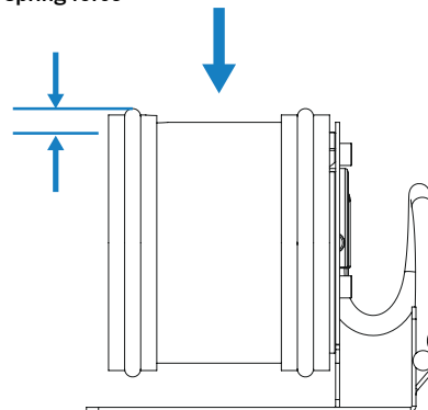
Figure 2: Working position / spring force = 2 ... 5 mm (5 ... 10 N)
