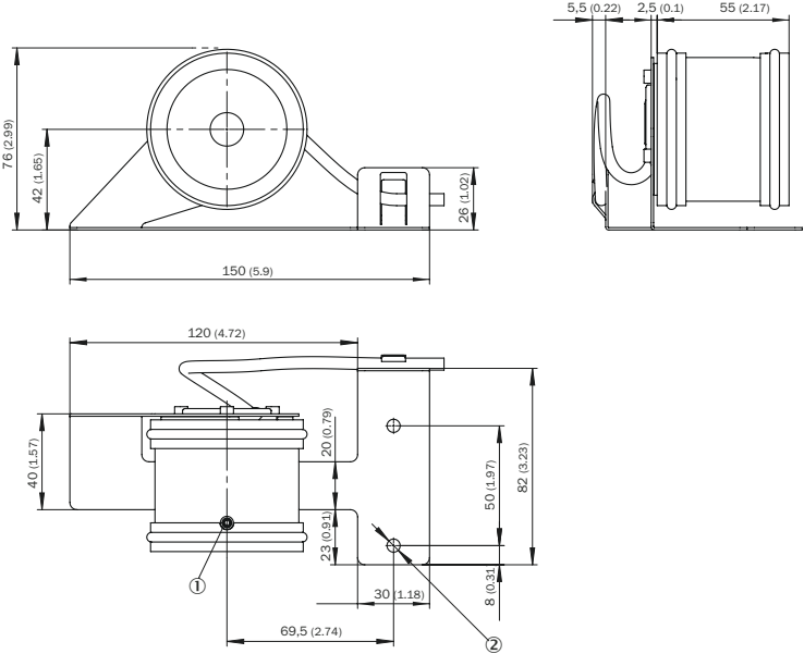
Figure 6: DKV60 with O-ring surface wheel ① M4 x 20 set screw ② 2 x Ø 5.5
