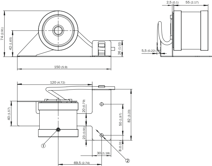
Figure 5: DKV60 with knurled surface wheel ① M4 x 20 set screw ② 2 x Ø 5.5 General tolerances according to DIN ISO 2768-mk.
