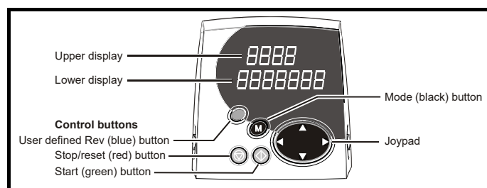
Figure 2-1 SM-Keypad
