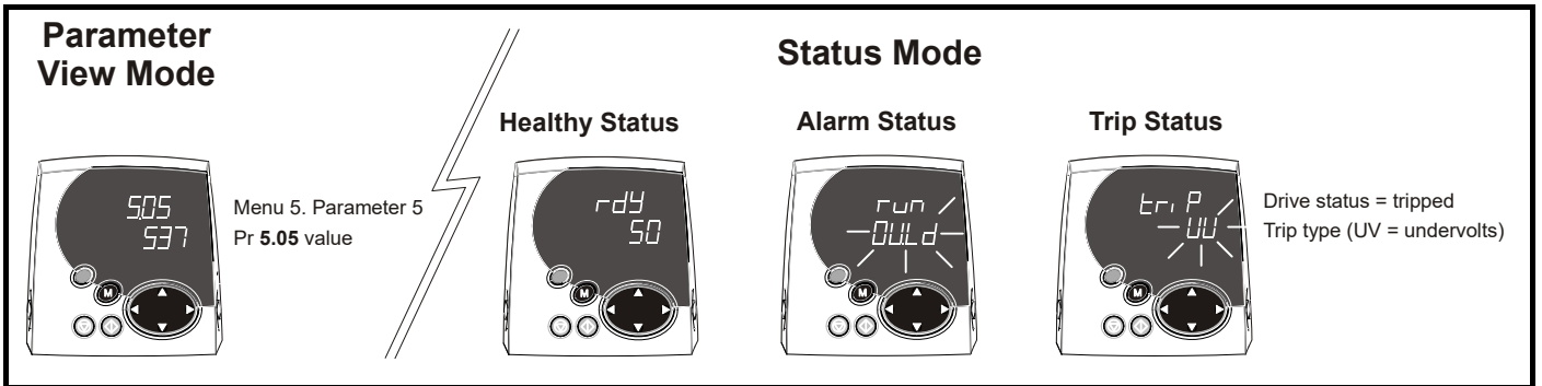
Figure 2-4 Mode examples
