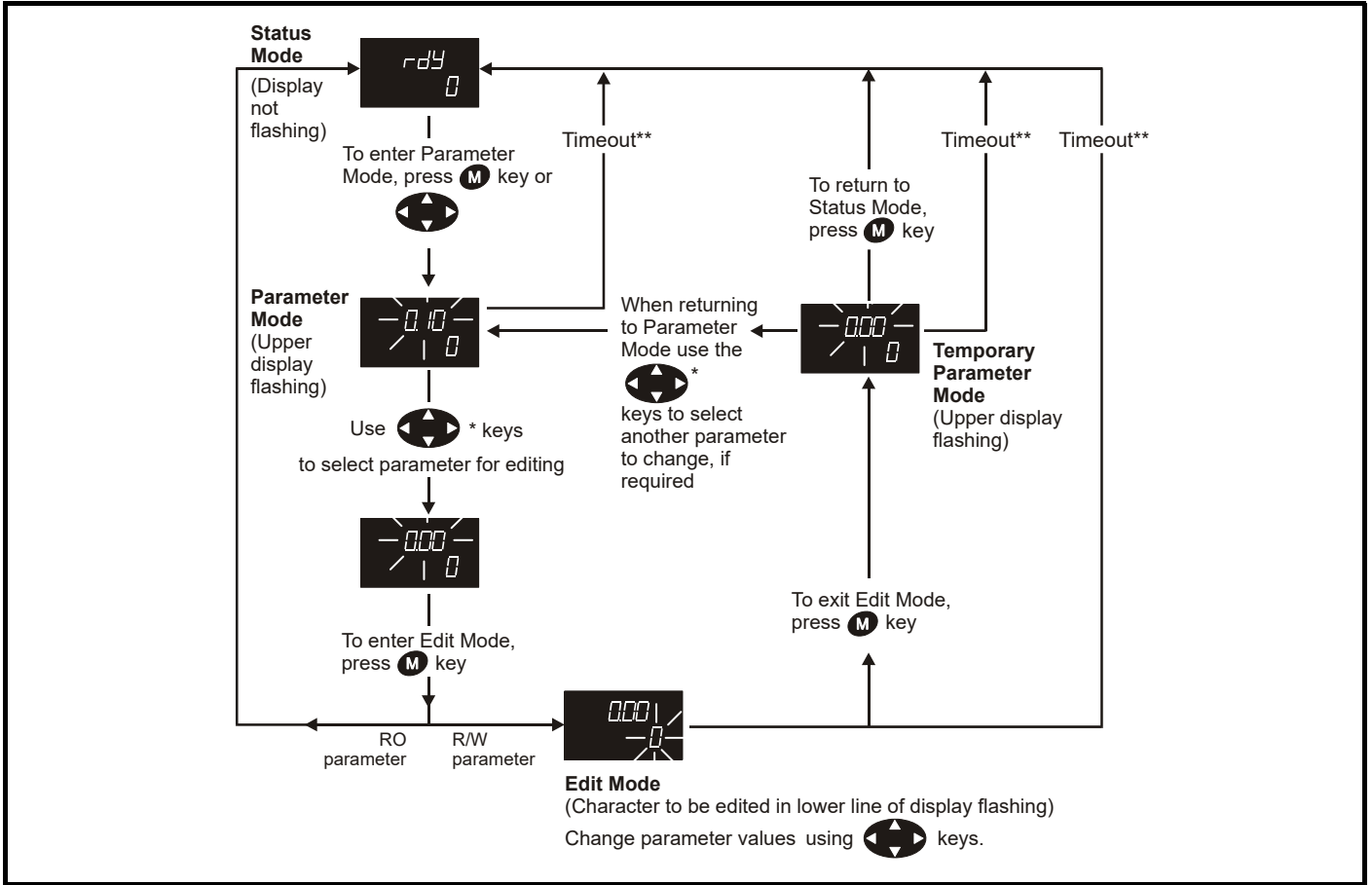
Figure 2-3 Display modes
