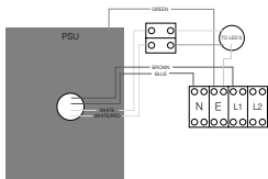
Typical wiring diagram - WL168-HO
