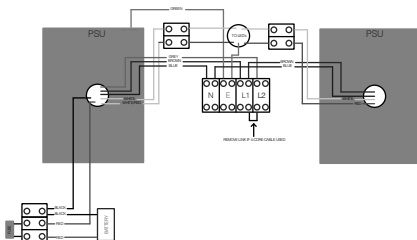
Typical wiring diagram - Emergency Variants
