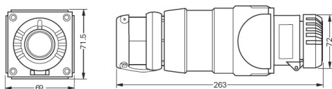
Coupler 3-pole
