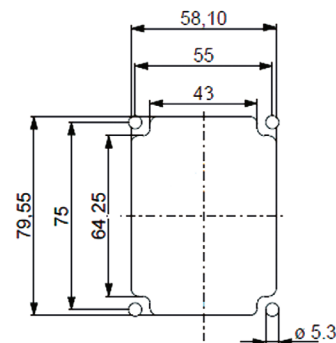
Angle adapter 16A 3-pol.
