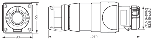
Coupler 4/5-pole
