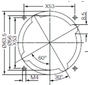
Assembly dimension
