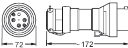
Plug 3-pole
