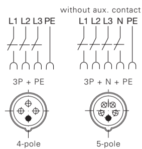
Plug 4/5-pole
