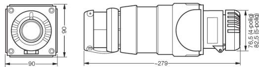
Coupler 4/5-pole
