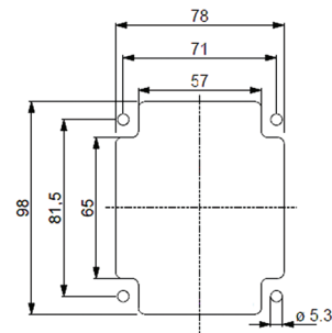
Angle adapter 16/32 A 4/5-pol.
