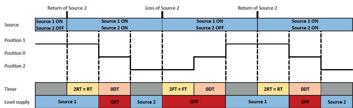
Loss and return of source 2 with source 2 priority
