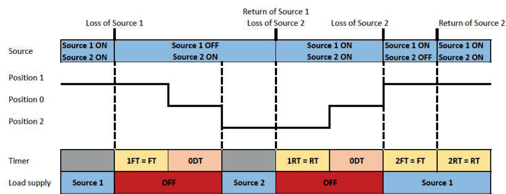
Loss and return of source 1 with source 1 priority
