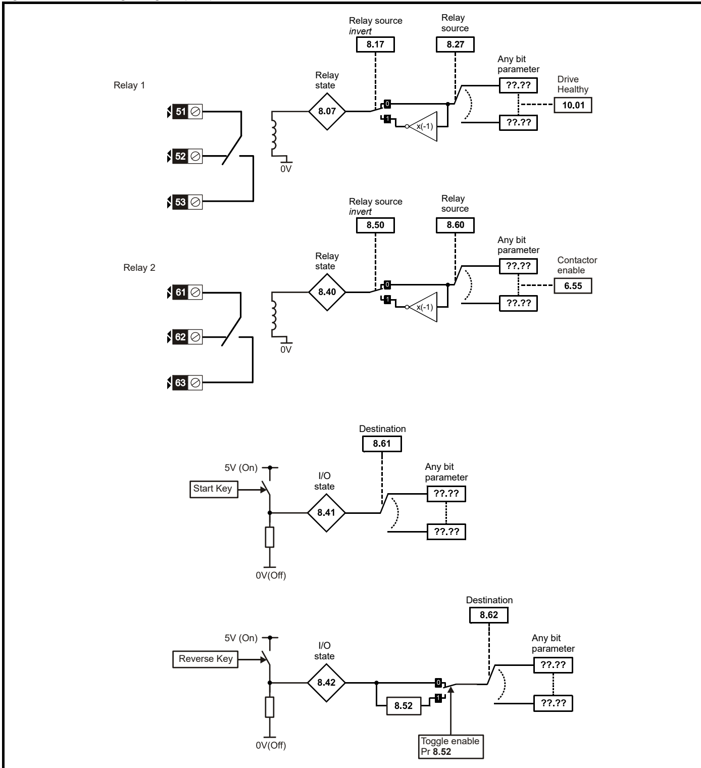
Figure 5-26 Menu 8 logic diagram (cont)
