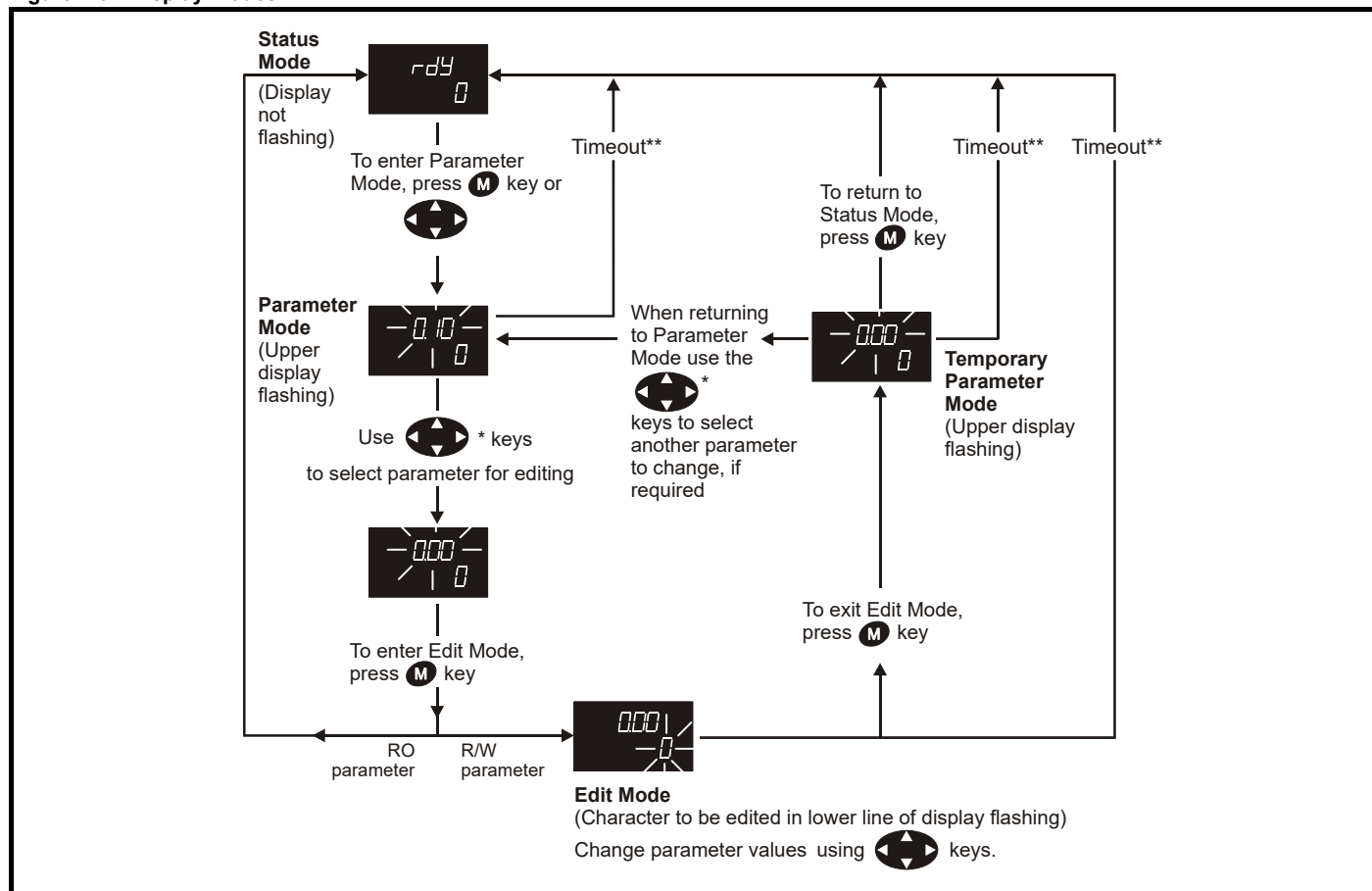
Figure 2-3 Display modes
