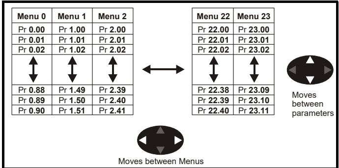
Figure 5-37 Menu structure
