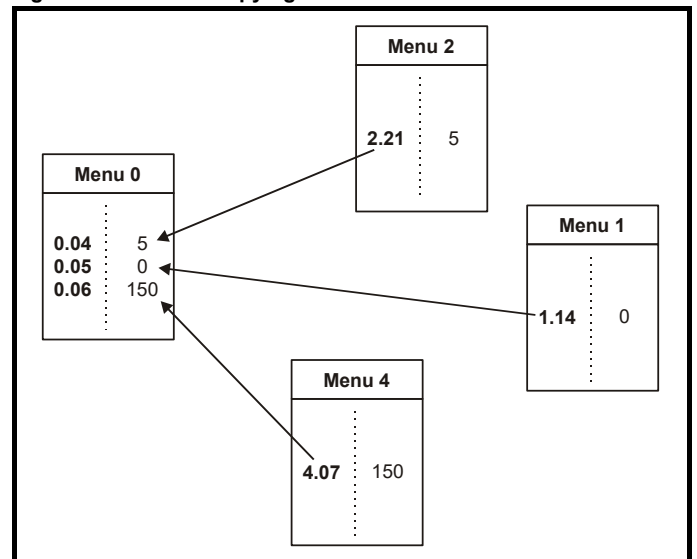
Figure 1-4 Menu 0 copying
