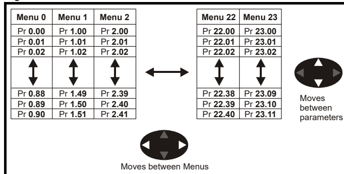
Figure 1-2 Menu structure
