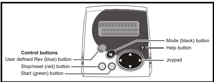
Figure 2-2 MP-Keypad
