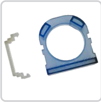
Holder for leakage sensors (LEAK) Article number 196329 Description H-D38-Leak-PVC
