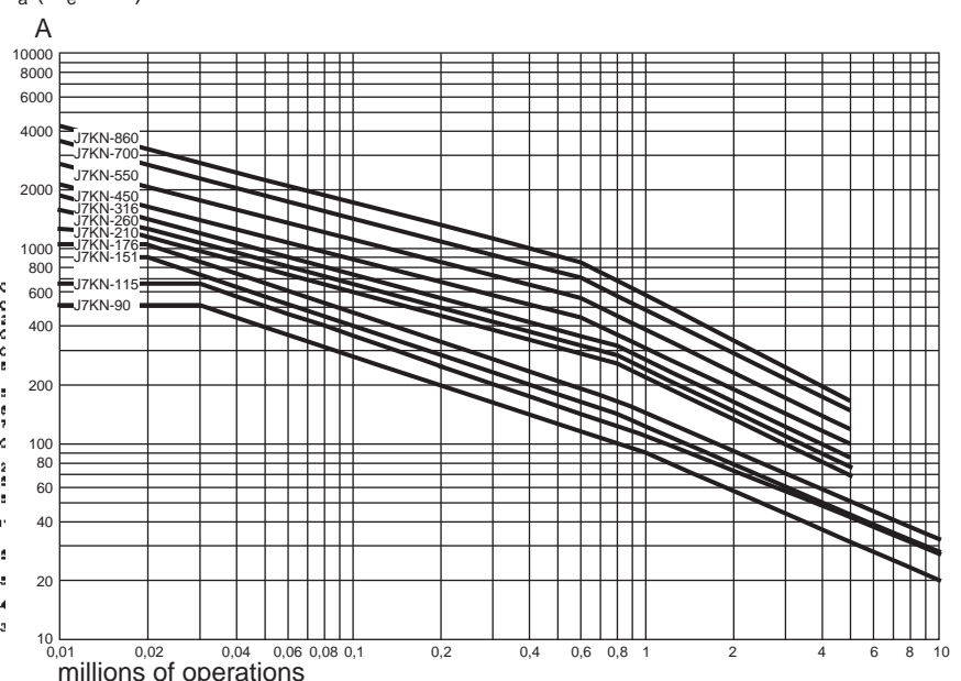
Breaking Current I_a (=I_e/AC1)
