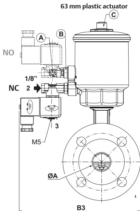
TYPE 02 Pilot 356, brass body Epoxy moulded IEC 335 / DIN 43650 / IP65
