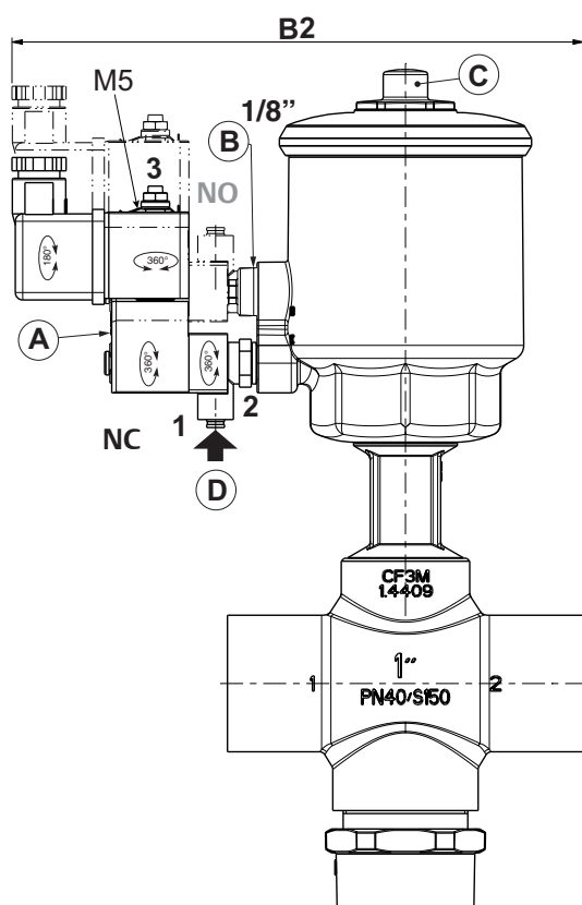
63 mm plastic actuator
