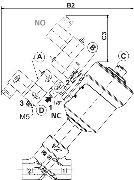
32 mm and 50 mm stainless steel actuators
