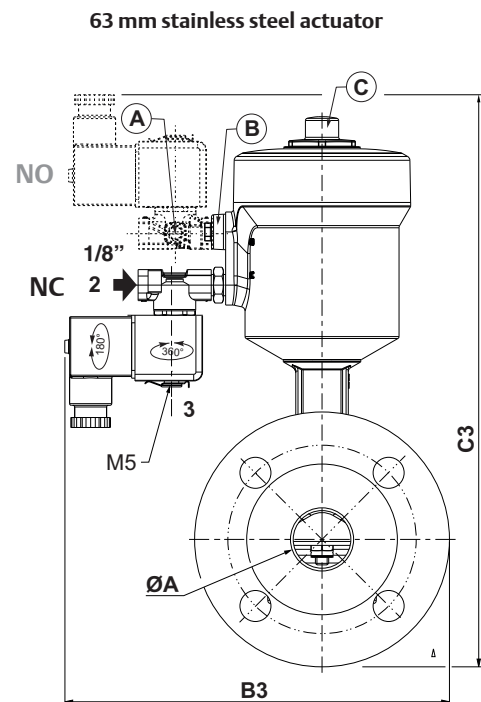
TYPE 02 Pilot 356, stainless steel body Epoxy moulded IEC 335 / DIN 43650 / IP65
